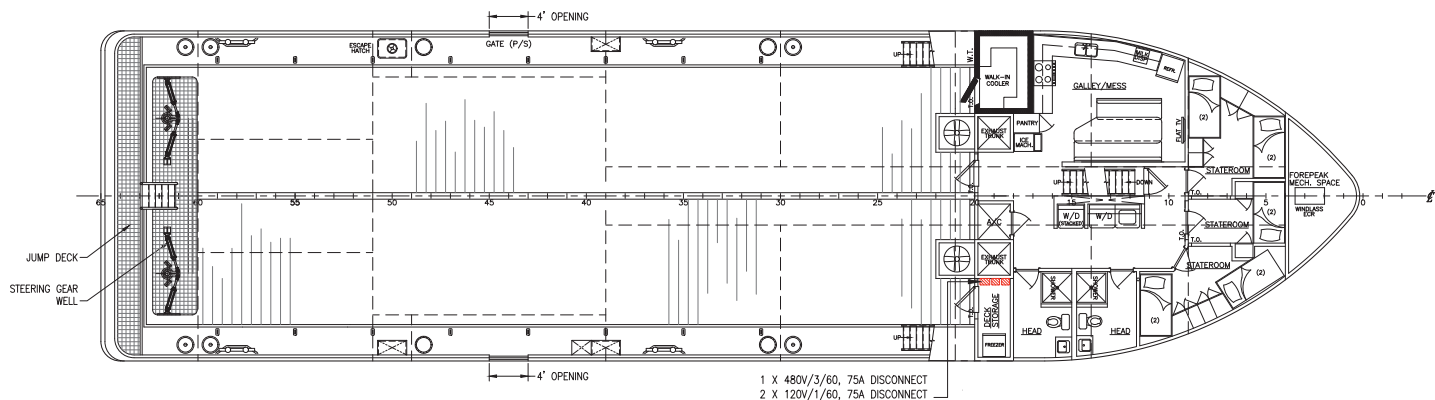
MAIN DECK
