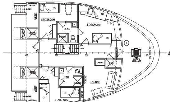
FOC'SLE DECK
