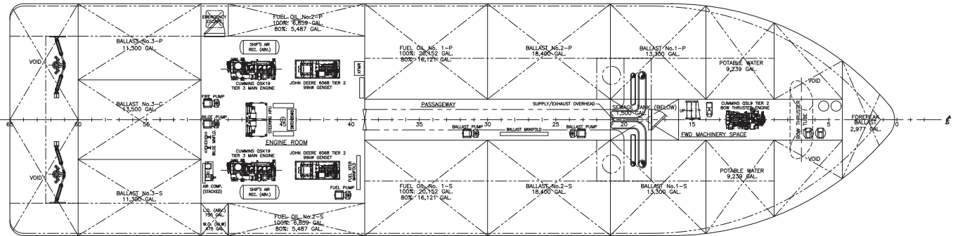
HOLD PLAN
