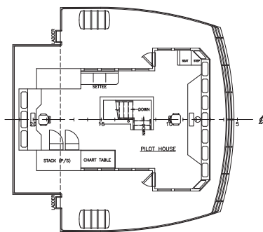
BRIDGE DECK
