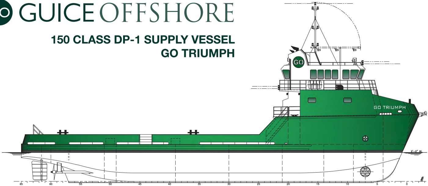
OUTBOARD PROFILE
