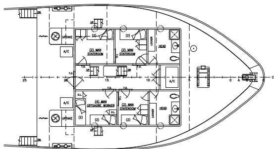
FOOSLE DECK
