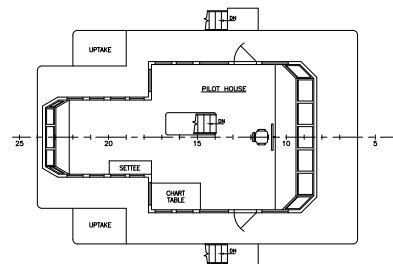
BRIDGE DECK
