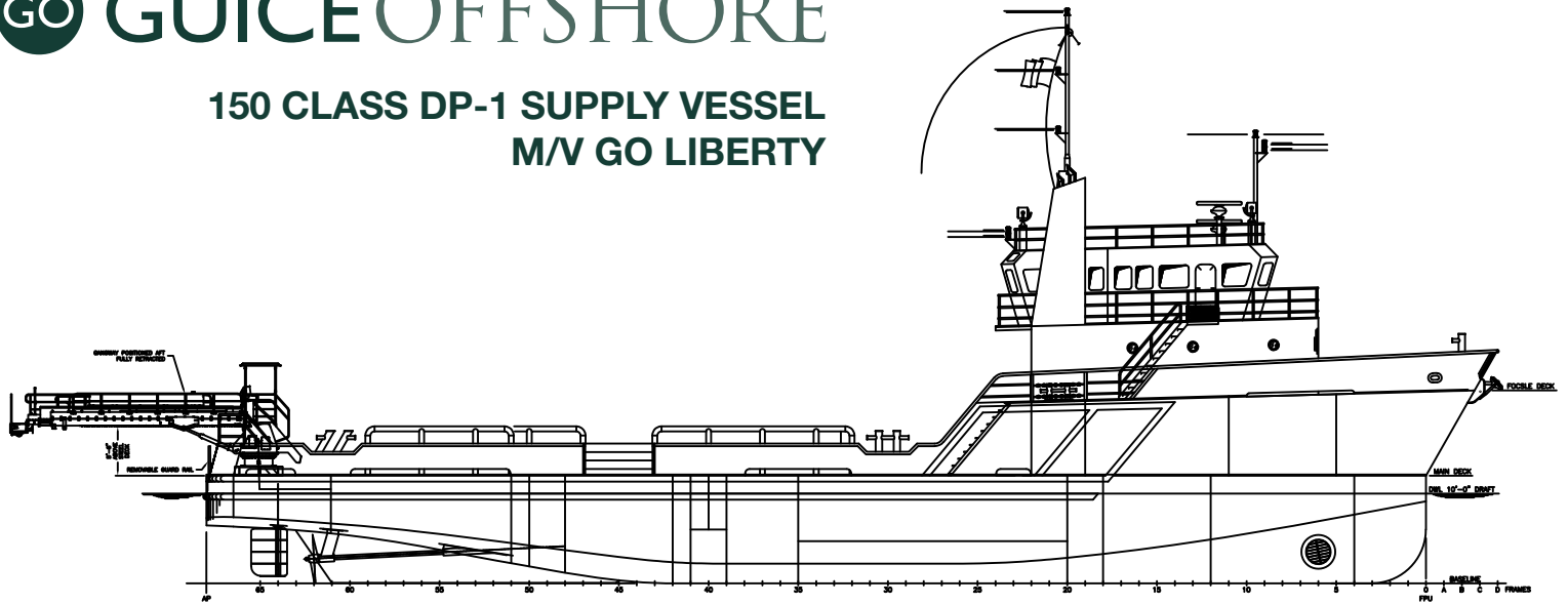
OUTBOARD PROFILE
