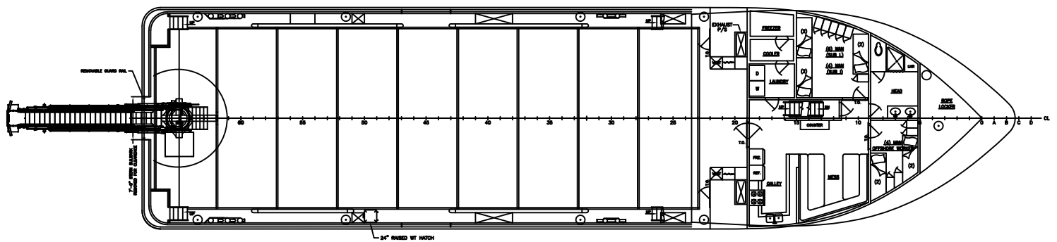
MAIN DECK
