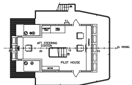
PILOTHOUSE ARRANGEMENT
