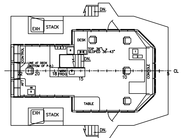
NAVIGATION DECK
