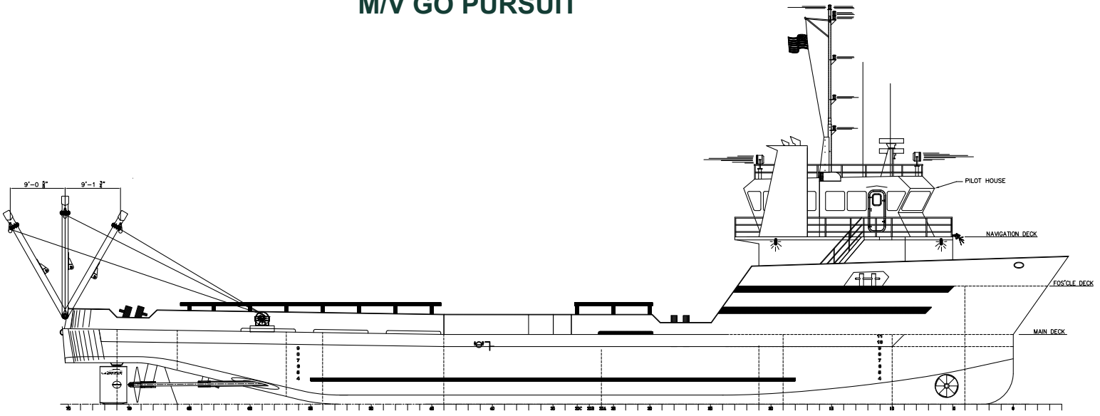
OUTBOARD PROFILE
