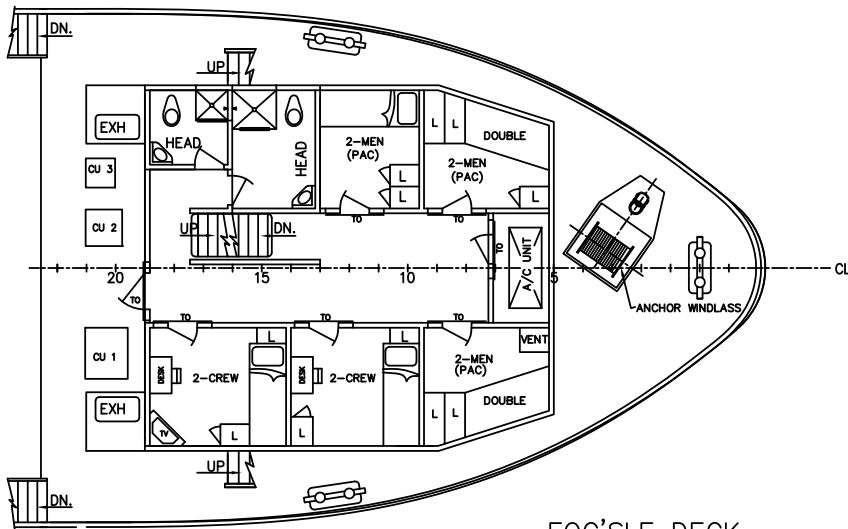
FOC'SLE DECK
