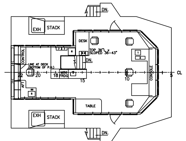
NAVIGATION DECK
